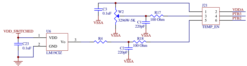
Temperature Sensor Circuit
