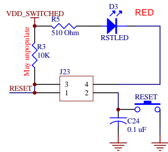
RESET CIRCUIT
