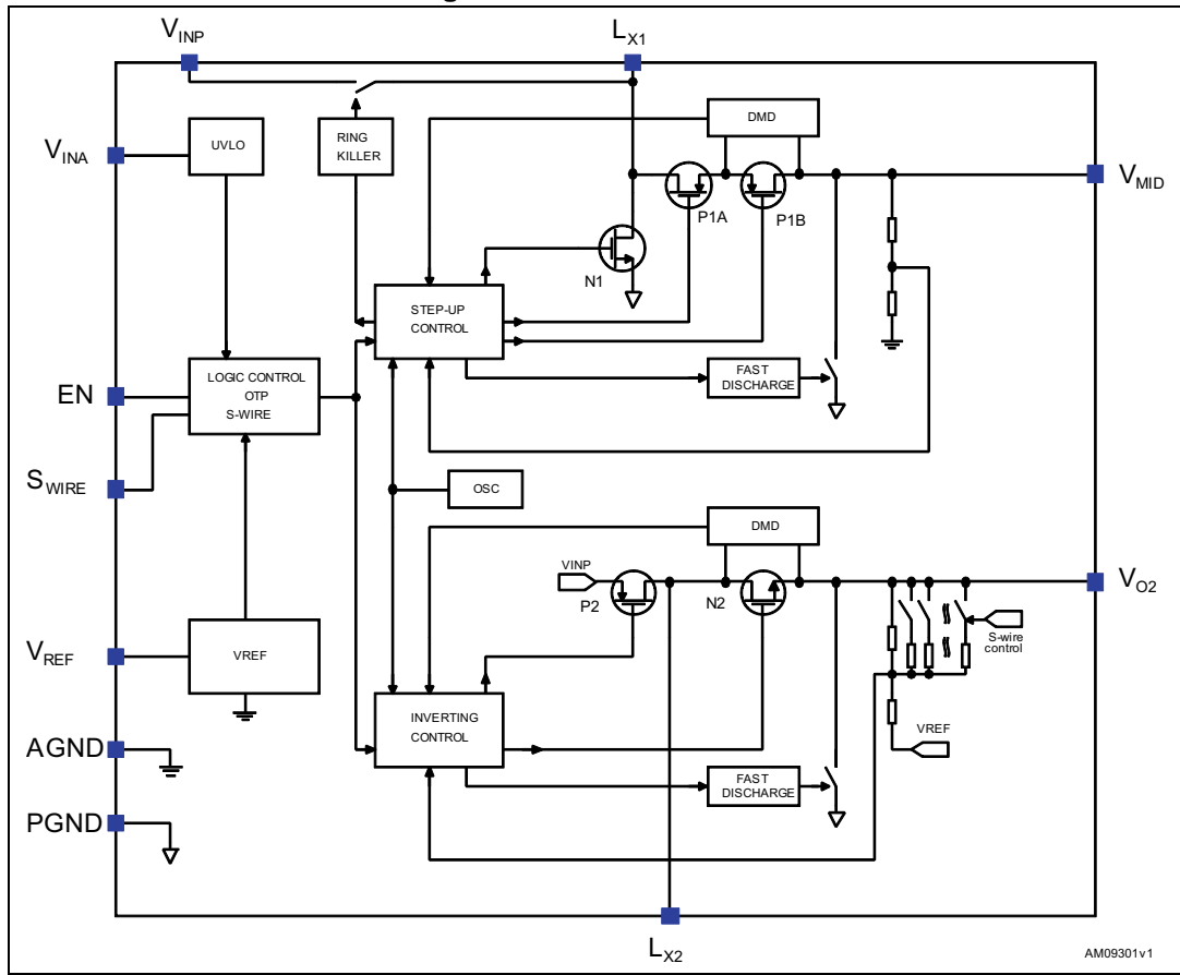
Figure 2. Block schematic
