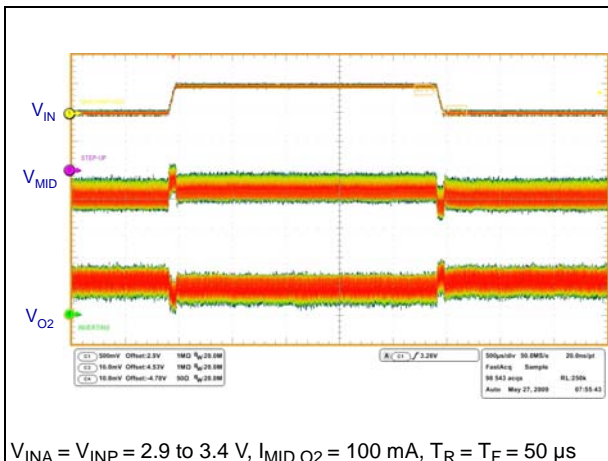
Figure 12. Line transient
